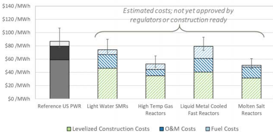
Figure 6: Estimated costs of SMRs and advanced nuclear reactors [ETI, 9]
